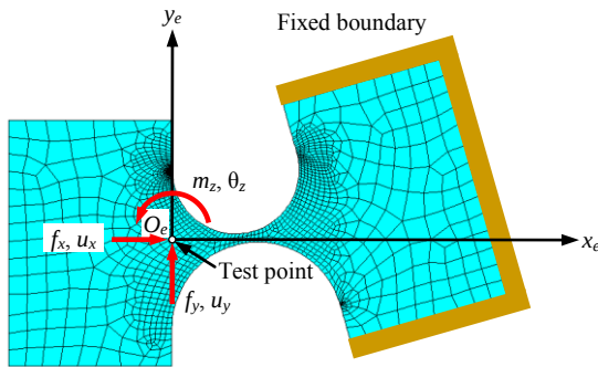
Fig. 5. Finite element model of the right circular flexure hinge prototype
