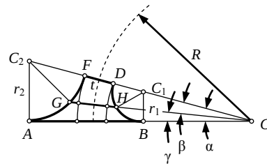
Fig. 4. Half of the circular-axis symmetric right circular flexure hinge with defining geometry
