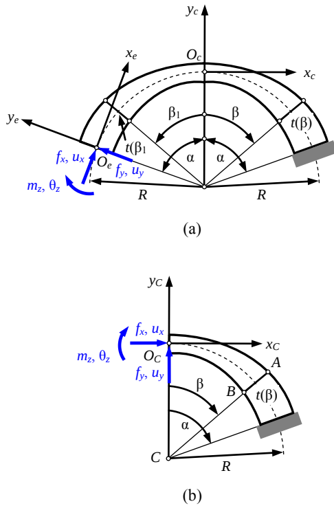
Fig. 3. (a) Symmetric circular-axis flexure hinge; (b) Half flexure hinge – both shown with end load and deformations
