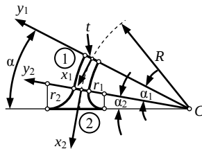
Fig. 7. Half of the circular-axis symmetric right circularly corner-filletted flexure hinge with defining geometry
