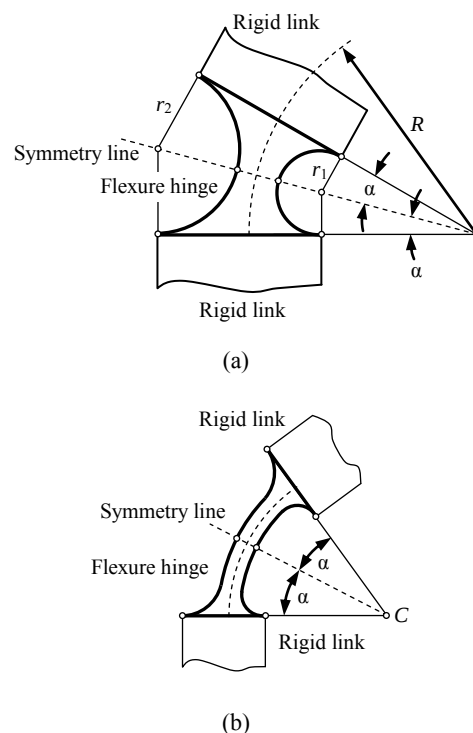
Fig. 2. Circular-axis flexure hinges: (a) Right circular; (b) Right circularly corner-filletted (radius of median circle is R )
