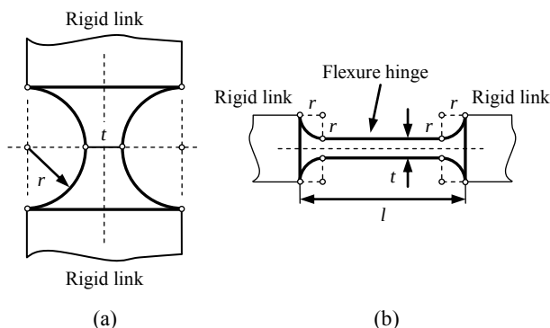
Fig. 1. Two common straight-axis flexure hinges: (a) Right circular; (b) Right circularly corner-filletted
